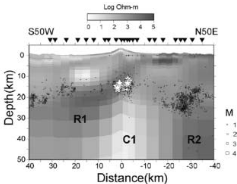
図 12 富士山の 2 次元比抵抗構造．構造の特徴的方向は，N 40 W と仮定している．三角印は観測点．1998 年から 2002 年までの 5 年間の震源を同時に示す．白丸は，鶴岡（1997）による構造的な地震，星印は，中道・他（2004 b）による低周波地震を示す． Fig .12 . Resistivity model obtained by 2 D inversion modeling of MT data 2 D regional strike direction ( parallel to the structure ) is assumed to be N 40 W . Inverted triangles indicate the measurement sites . Seismicity for 5 years ( 1998 2002 ) in a swath of 20 km wide is also plotted . Earthquake magnitude is shown on right . Open circles indicate tectonic earthquakes ( Tsuruoka ,1997 ) . Stars show locations of 76 low frequency earthquakes which were recorded with good signal to noise ratios ( Nakamichi et al . ,2004 b ) .
