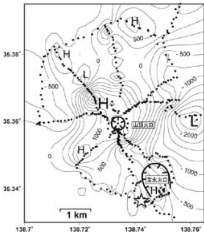
図 10 富士山山頂周辺における自然電位分布．線の間隔は 0.25 V．星印は，観測の基準点，太線は，山頂および宝永の火口を示す． Fig .10 . Self potential distribution around the summit of Fuji Volcano . Contour interval is 0.25 V . Star shows the reference point . Thick lines indicate the locations of the summit crater and the Hoei crater .
